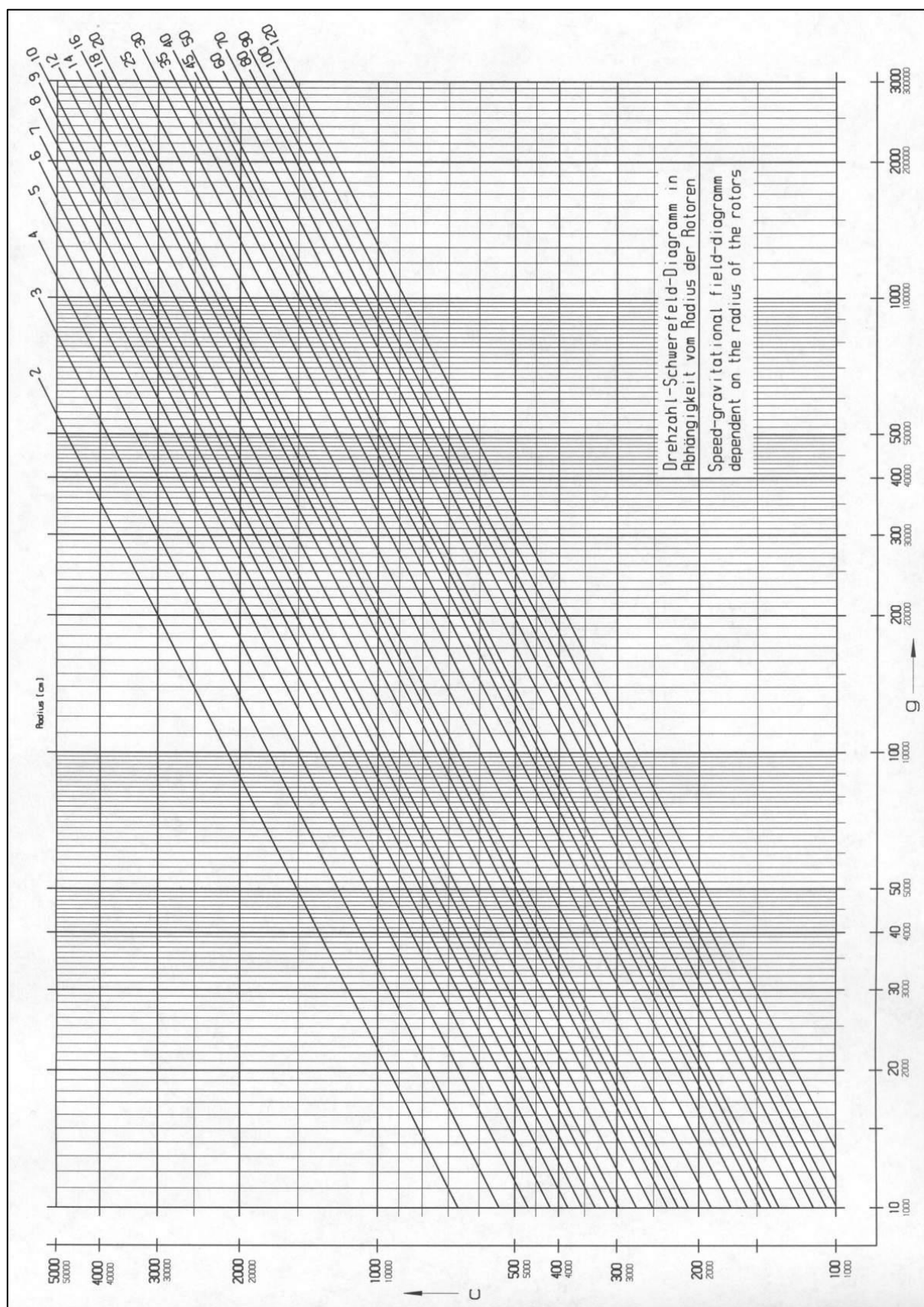
Fig. 41: Speed-gravitational-field-diagram
